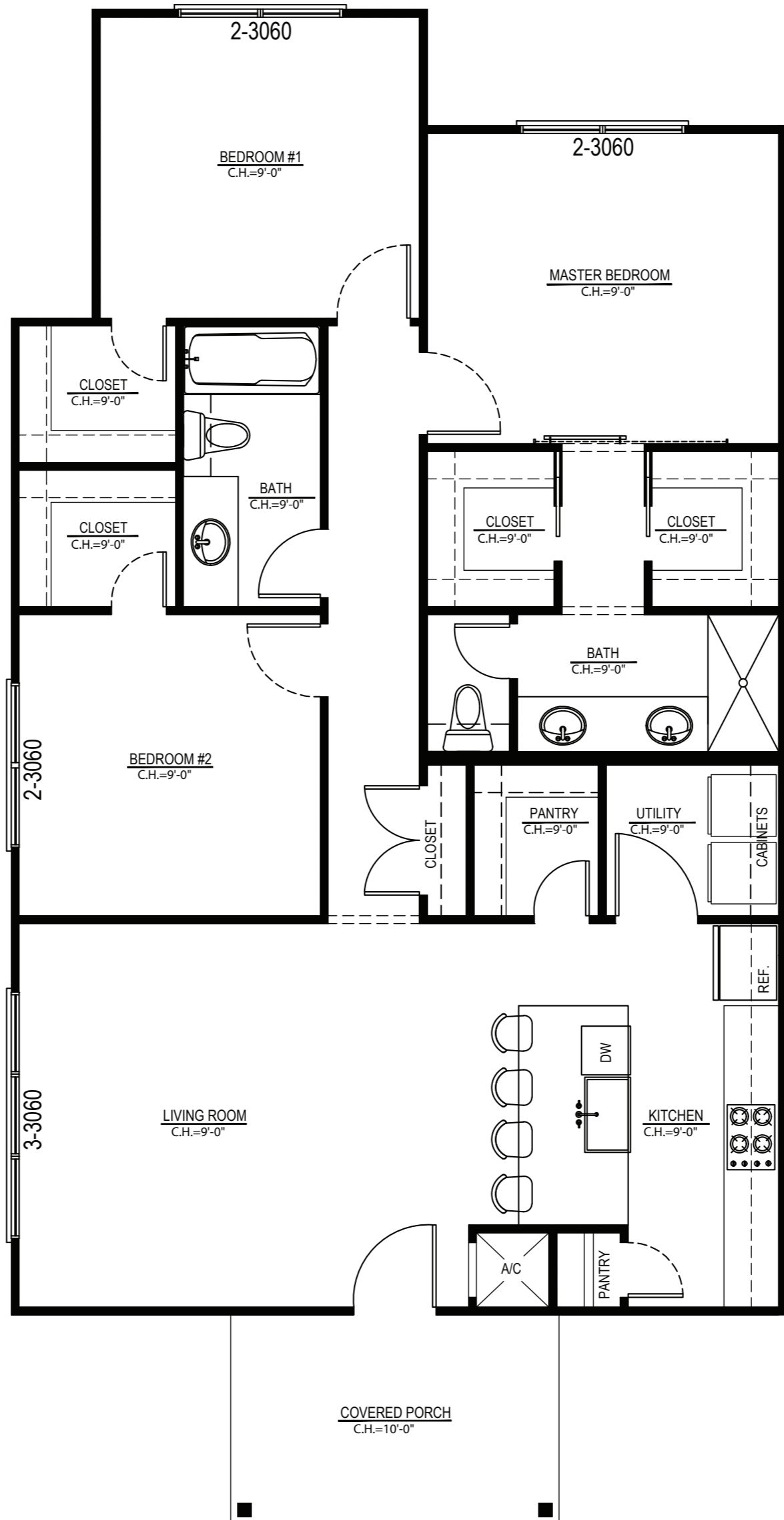
Three Bedroom & Two Bathroom Floorplan
